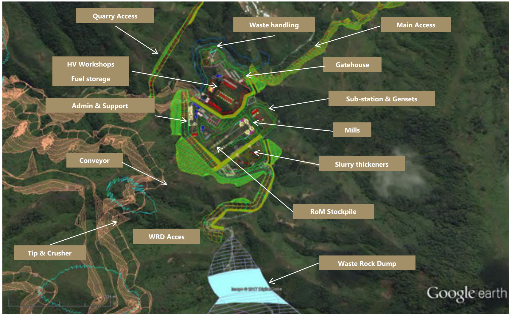
Figure 18-3: Yandera Mining Precinct
